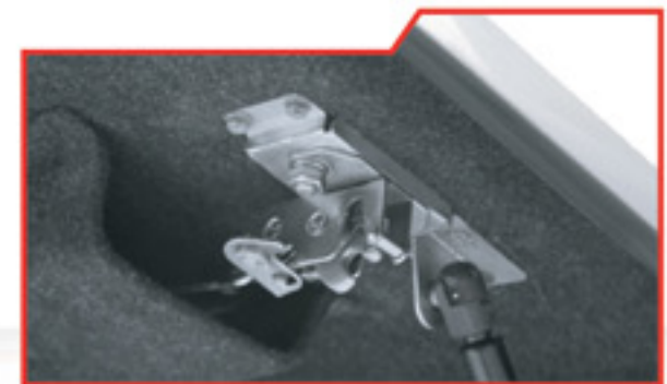
Rotary lock and latch
